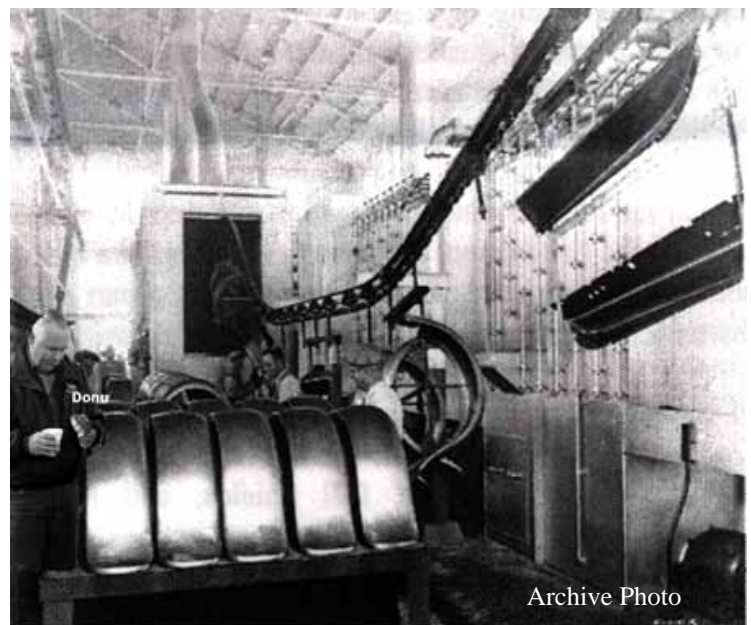
Jim watches his fenders being prepared for the paint conveyor
